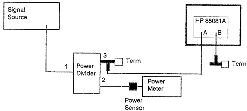
Figure 5-2. SRD Bias Adjust Setup
