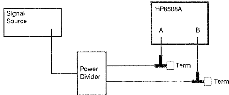
Figure 5-17. LF Phase Adjust Setup
