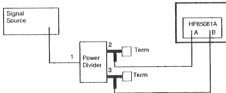
Figure 5-6. Delay Line Adjust Setup
