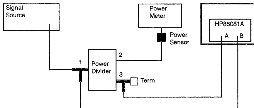
Figure 5-9. Channel Gain Setup
