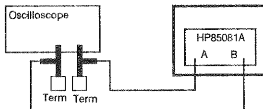
Figure 5-7. Symmetry Adjust Setup
