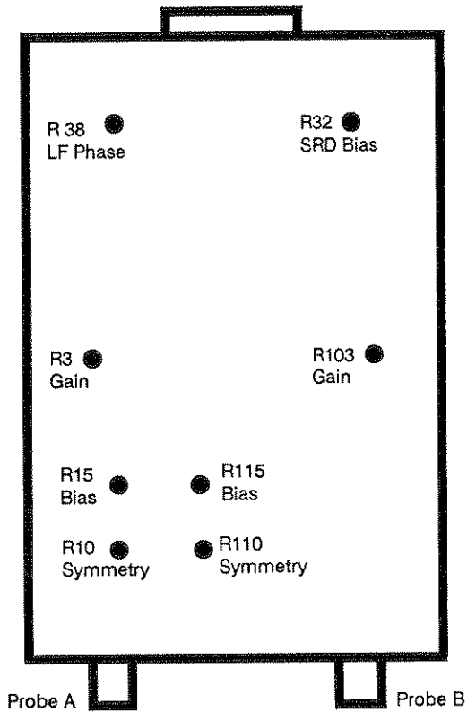
Figure 5-16. Input Module Adjustment Locations
