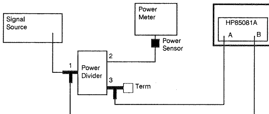
Figure 5-4. Bias Adjustment Setup
