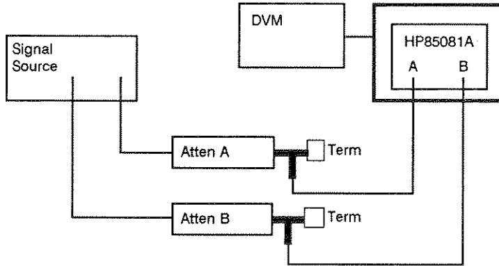
Figure 4-7. Amplitude Accuracy vs Input Level (and rear panel output check) Test Setup
