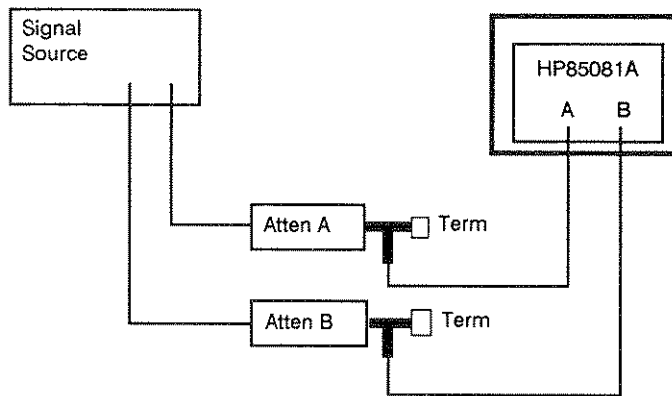
Figure 4-8. Voltage Ratio Accuracy Test Setup
