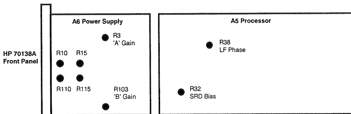
Figure 5-1. Input Module Adjustment Access Points in the HP 70138A
