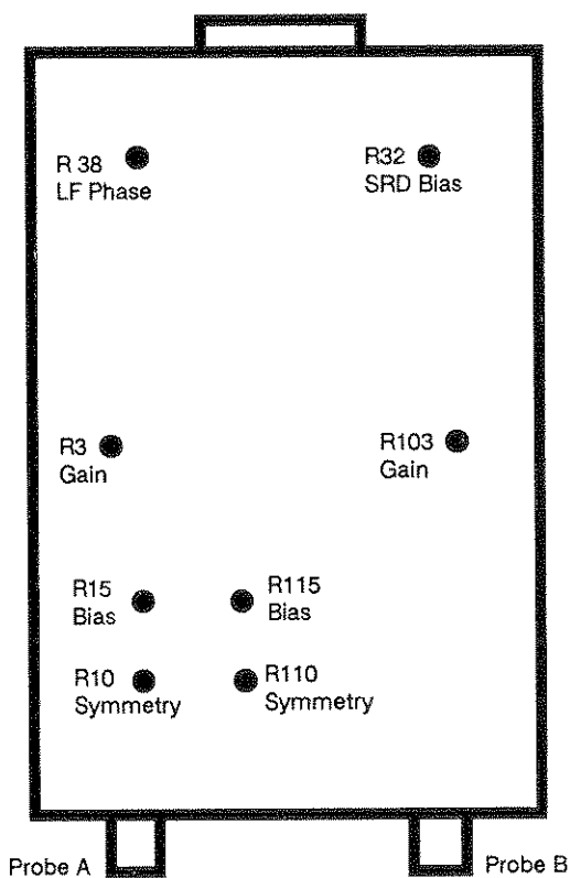
Figure 5-14. Input Module Adjustment Locations
