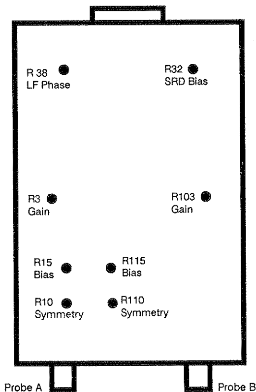
Figure 5-18. Input Module Adjustment Locations
