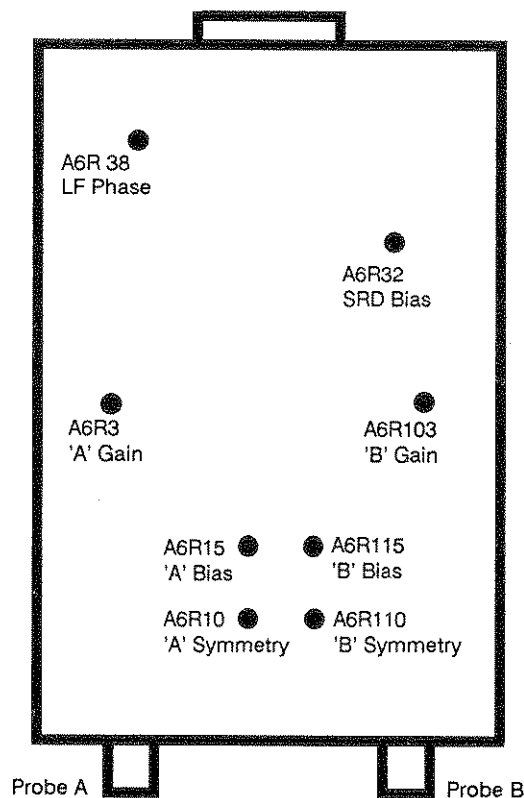
Figure 5-12. Input Module Adjustment Locations
